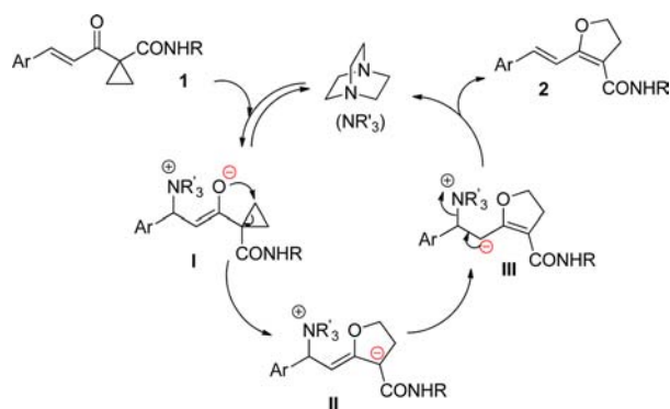
Scheme 3. Proposed Organocatalyzed Anion Relay Mechanism
