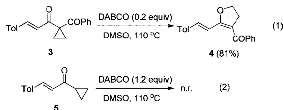
Scheme 2. Further Scope Extension
